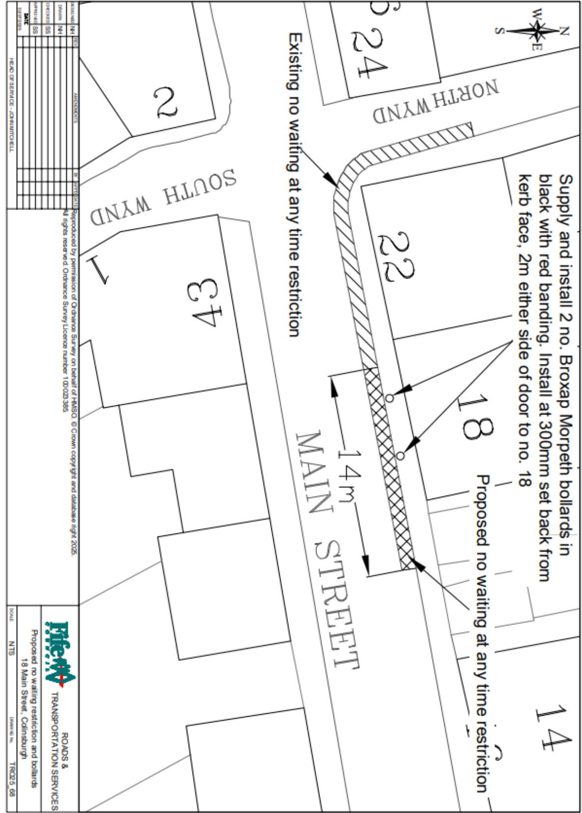
Picture caption: Plan showing proposed extension to no waiting at any time restriction at Main Street, Colinsburgh
