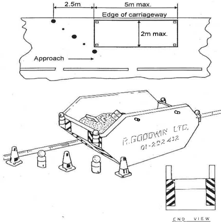
Figure 1. ARRANGEMENTS FOR SITING A SKIP
